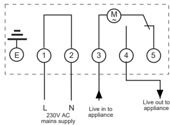
OP-SBSDIGI Installation
