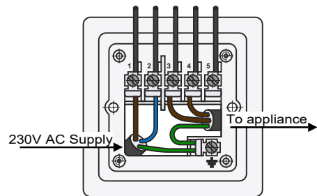
Wiring diagram (Volt Free)
